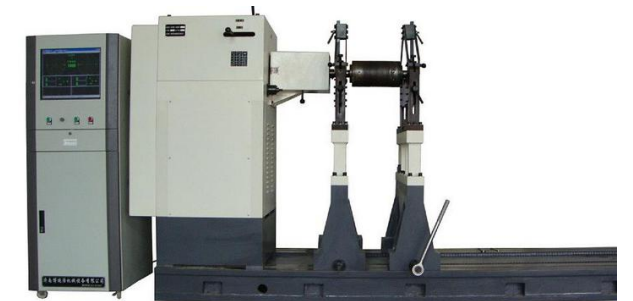
Horizontal Dynamical Balance Testing Instrument
